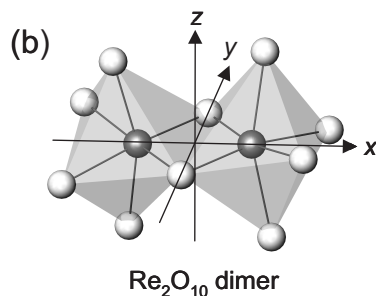
Figure 8(b). Definition of the Re d-orbital directions following that in [16].
